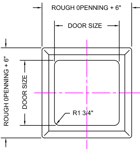
Drop-in Access Panel -Type Panel Elevations
